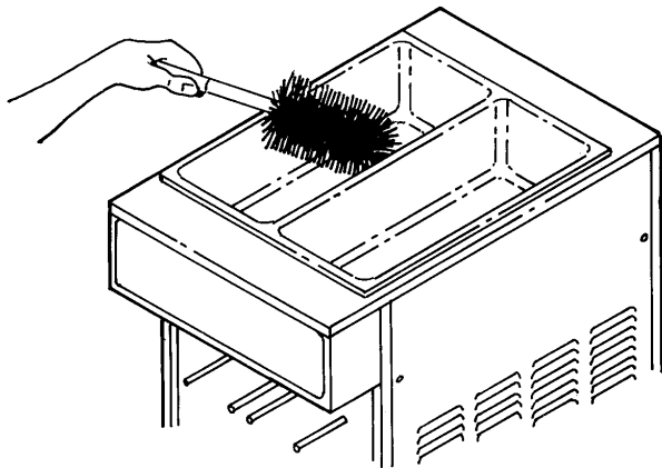
Figure DD Sanitize Hopper
